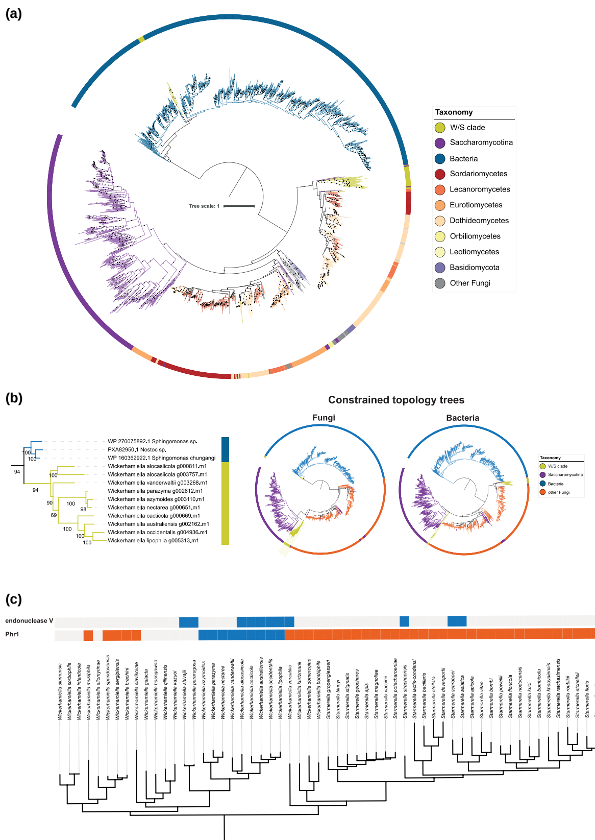
Fig. 4. Several W/S-clade species acquired bacterial DNA repair genes through horizontal gene transfer (HGT). (a) Phylogenetic tree of sequences with the highest sequence similarity to Phr1 from Wickerhamiella australiensis and Starmarella bombycola . Branches are colored according to taxonomy (species outside Dikarya or Pezizomycotina species for which no taxonomic class could be determined were categorized as "Other Fungi"). (b) (on the left) Pruned Phr1 phylogeny depicting the HGT event from bacteria (Sphingomonadales) to a W/S subclade. On the right, the resulting trees from the constrained topology analyses are shown: Fungi—constrained topology considering monophyly of the W/S Pezizomycotina-like sequences and other Saccharomycotina (excluding the Saccharomycotina sequences that cluster with other Fungi) and Bacteria—constrained topology considering monophyly of bacteria-like W/S sequences and Saccharomycotina sequences (excluding those clustering with other fungi). (c) Distribution of putative HGT-derived (blue: bacterial, orange: fungal) PHR1 and endonuclease V genes across the W/S clade. Original tree files and sequence alignments can be found in Figshare ( https://figshare.com/s/3d575d6283c970a0c1e4 ).
